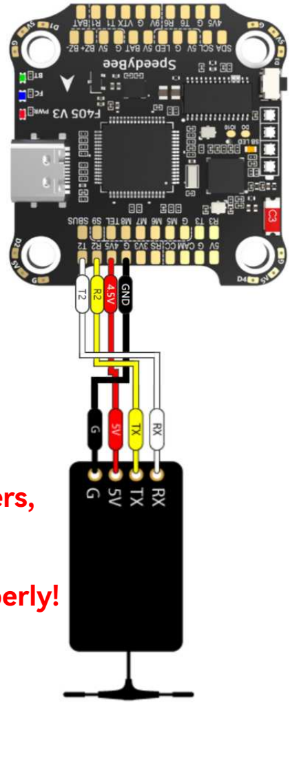
ELRS Receiver
