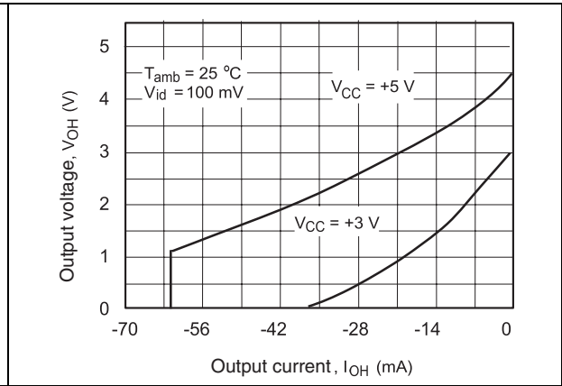
Figure 3. High level output voltage vs. high level output current (VCC = +5 V, VCC = +3 V)
