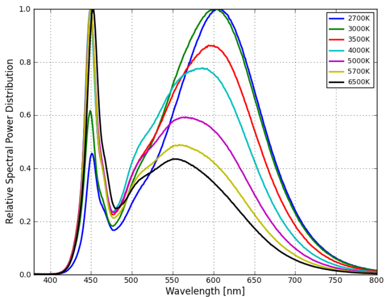
Figure 2. Emission color spectrum for MXZx-PWXX.
