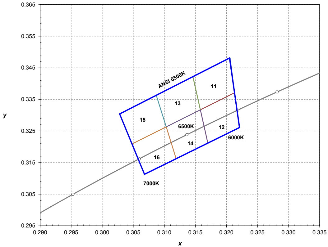
Figure 17. ANSI 6500K 1/6th color bin structure, forwards current = 30 mA, thermal pad temperature = 25°C.
