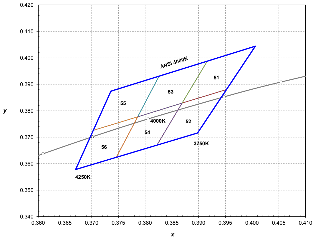
Figure 14. ANSI 4000K 1/6th color bin structure, forwards current = 30 mA, thermal pad temperature = 25°C.
