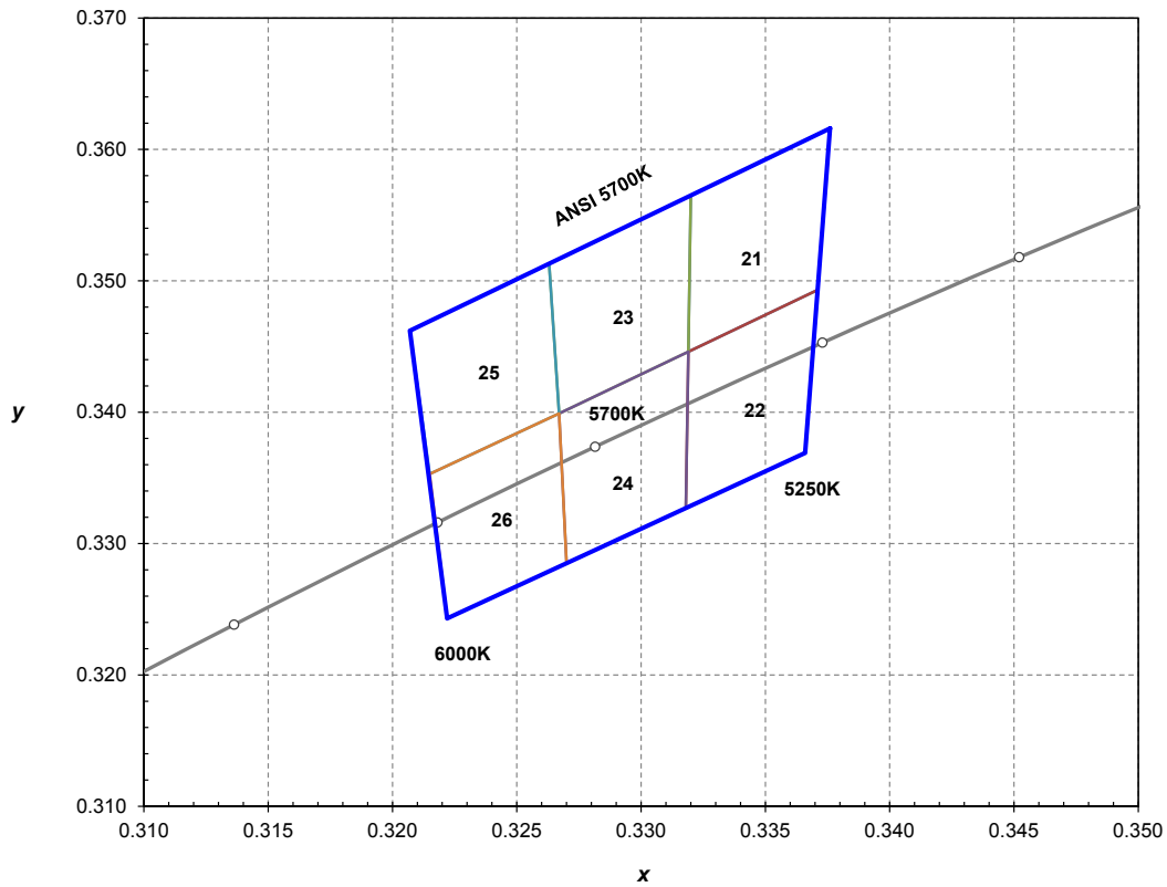
Figure 16. ANSI 5700K 1/6th color bin structure, forwards current = 30 mA, thermal pad temperature = 25°C.
