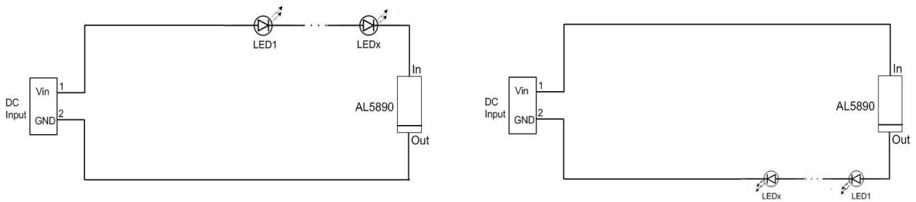
(DC Configuration)
