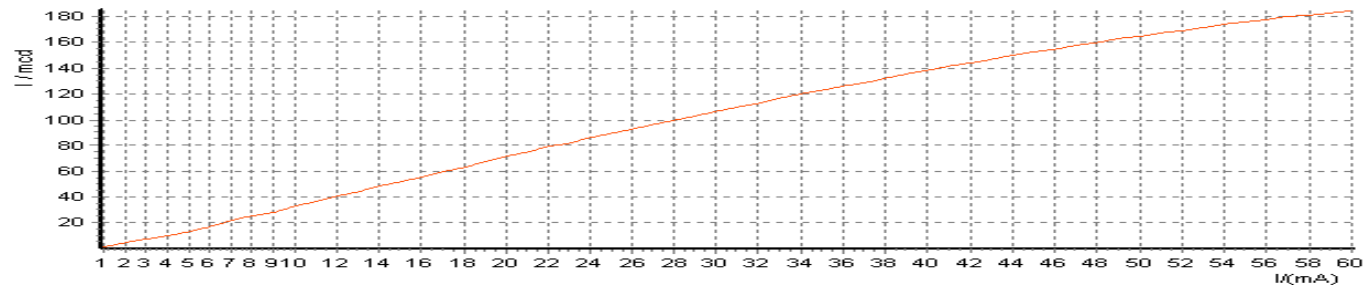
Current-Luminous intensity Curve
