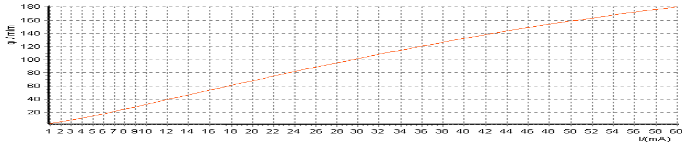
Current-Luminous flux Curve
